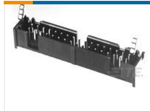
TE Part #1-1761608-5 IDC LOW PRO HDR 50P VERT SHT L
