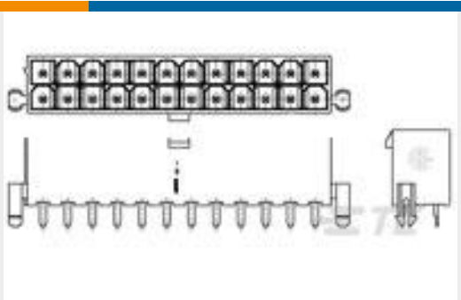
TE Part #1-1586040-2 12P VAL-U-LOK VRT HDR W/P V0
