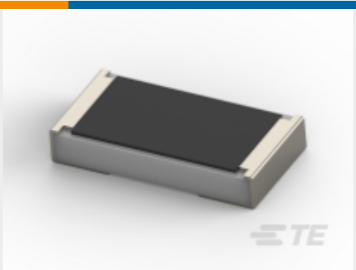
TE Part #1-2176232-6 SMD Power Resistor: 3 Watt, 1% Tol
