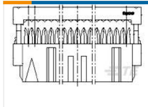
TE Part #1-215919-6 AMP-LATCH 15.2 HIGH TAPE
