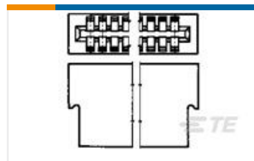
TE Part #1-583717-3 TW LEAF CRP HSG. 30-POS.
