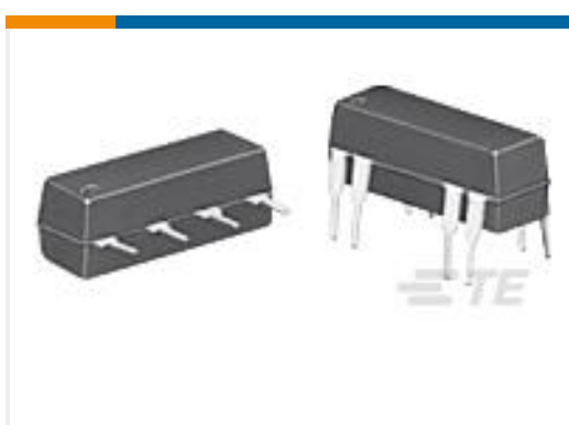
TE Part #1-1393771-1 JWD-171-17=REED RELAYS
