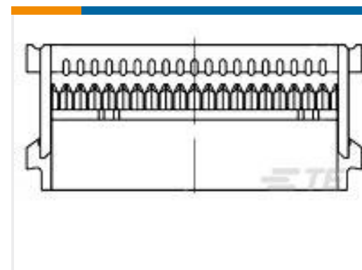
TE Part #1-1658526-8 609-3430LF FEM SOCKET, LEAD FREE
