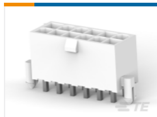
TE Part #1-2825261-2 12P VAL-U-LOK HCS VRT HDR W/P V0
