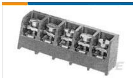
TE Part #1-1437652-3 6PCR-12-006=#6 TRIBARRIER
