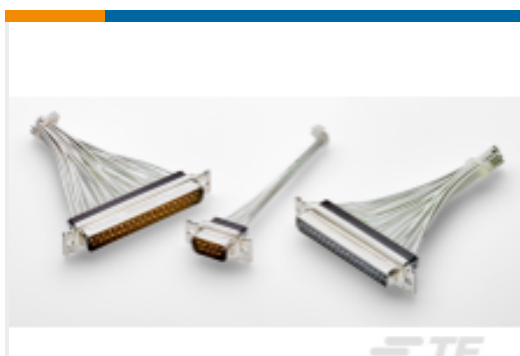
TE Part #2335893-2 AMPLIMITE SZ 2 RECPT 26 POS, ST STL SHEL
