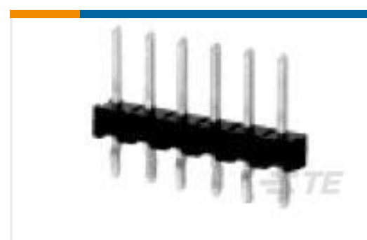
TE Part #104344-5 07 MODII HDR SRST B/A W/HD
