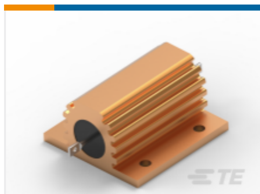
TE Part #1-1625984-0 Power Resistors: Aluminum Housed, HSA
