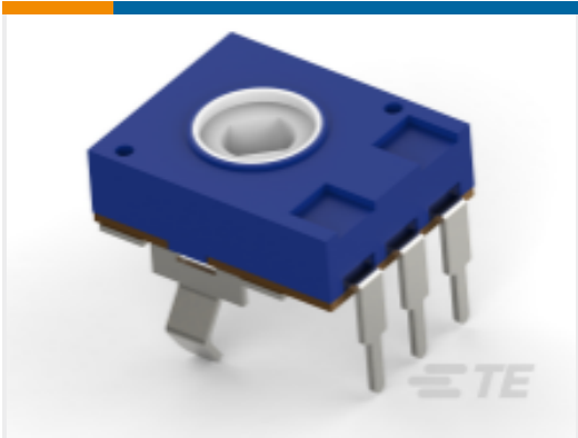
TE Part #2176394-2 51T 1K0 20% LINEAR 10K MOQ
