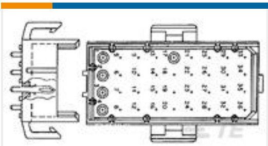
TE Part #1318699-5 MR HDR ASSY 24P COATING
