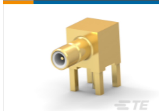
TE Part #1060442-1 SMB RF Connector: Male (Jack), Snap Fit, 50 Ohm
