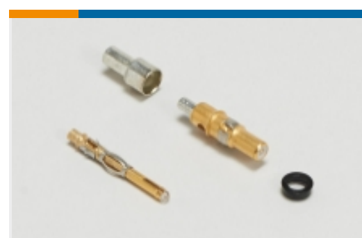
Coax Contacts(1)
