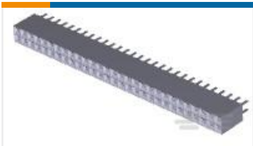
TE Part #2-535542-9 58 MODIV VRT DR CE 100/130
