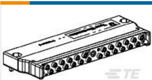
TE Part #1738960-2 CONNECTOR ASY,MODULE,24 POS, ARINC 801
