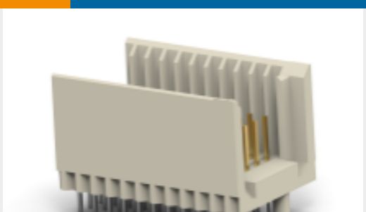
TE Part #100668-1 Hard Metric Male Connector: Traditional Backplane, Mezzanine, 2mm
