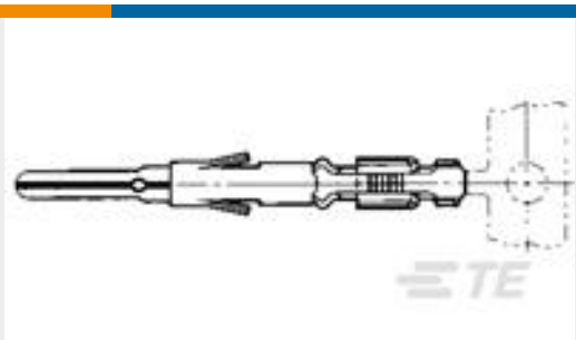
TE Part #203816-4 PIN CONTACT ASSY,L/P
