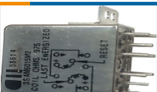
TE Part #4-1617522-1 3SAT1309A2=M5757/13-092
