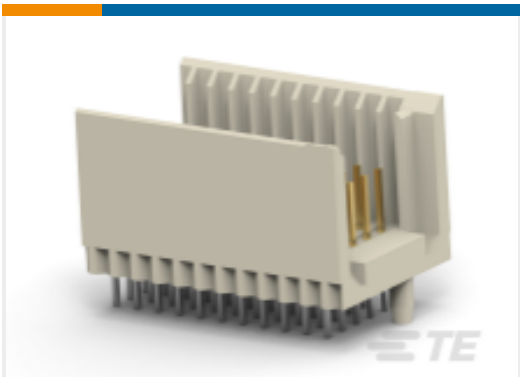
TE Part #5352128-1 Hard Metric Male Connector: Traditional Backplane, Mezzanine, 2mm
