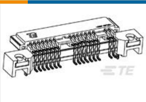
TE Part #1-1735583-1 mSATA, Receptacle, R/A SMT, Btm Mt, 30u"
