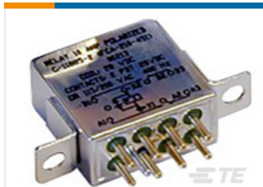
TE Part #1-1617784-5 FCA-210-1006M=M83536/10-006M
