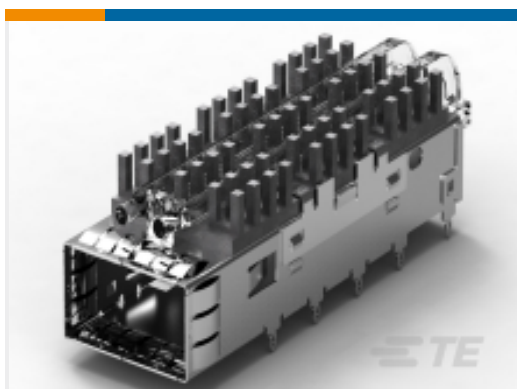
TE Part #2-2170705-8 CAGE ASSY, QSFP28 1X1, SPRING, HS, LP
