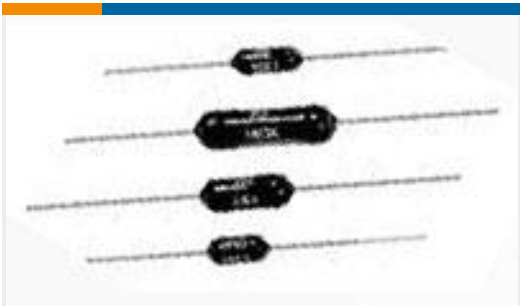
TE Part #2-1879673-3 H8 182R 0.1% 25PPM
