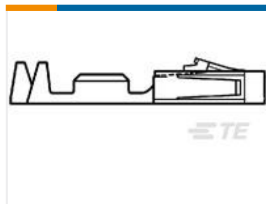
TE Part #104481-7 SHORT POINT RECP CONT LP
