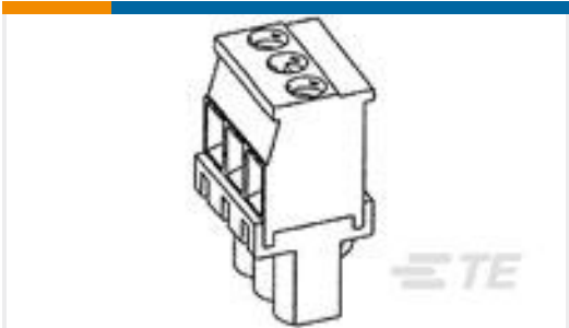
TE Part #1-1986375-3 Str Plug, 3.81mm, Green, LH, 13 posn
