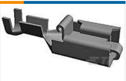
TE Part #154717-7 PL 250 REC TERMINAL 13-11 AWG PTPPB
