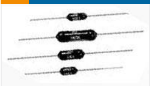
TE Part #1-1879622-8 H4P 680K 1% 50PPM
