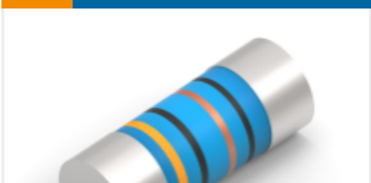
TE Part #5-2176315-6 MELF SMA_A 3K3 1% 50PPM 0204 0.4 W
