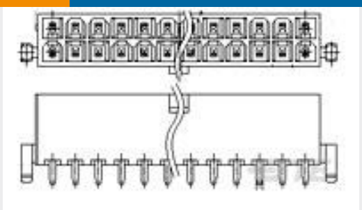
TE Part #2-1775099-1 ATX PWR CONN 2 BDLK 6 POS
