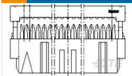
TE Part #1-215919-4 AMP-LATCH 15.2 HIGH TAPE
