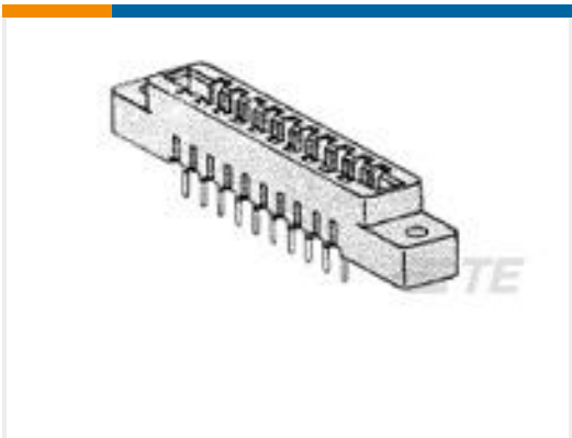
TE Part #2-530655-5 CONN LOW PRO 18 POS 156X200C/L
