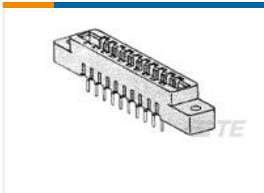
TE Part #2-530655-5 CONN LOW PRO 18 POS 156X200C/L
