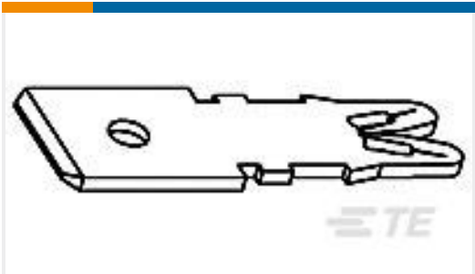
TE Part #4-1601006-2 031-015-002=TAB,187X020,STD SMZ
