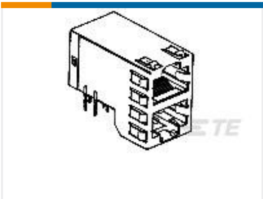
TE Part #6368168-5 2X1 OFFSET ST/JK,LED(G&Y)12PNL
