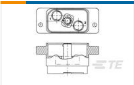
TE Part #1604896-2 ASY,RCPT,PWB MT,2 POS
