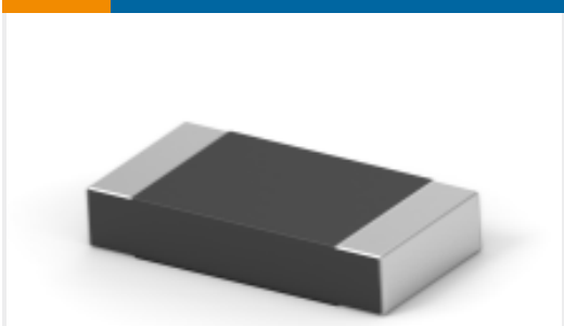
TE Part #1-1625827-0 Metal Chip Resistor: Current Sense
