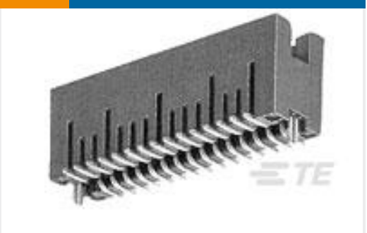
TE Part #1-104656-0 100 50/50 HDR DRST SFMNT .320
