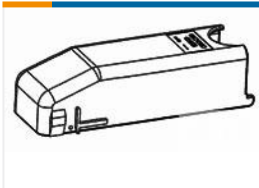
TE Part #1393454-6 V23542C1052Z100=52P COVER
