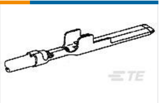
TE Part #170221-3 TAB WITH LANCE FOR M.I.C.
