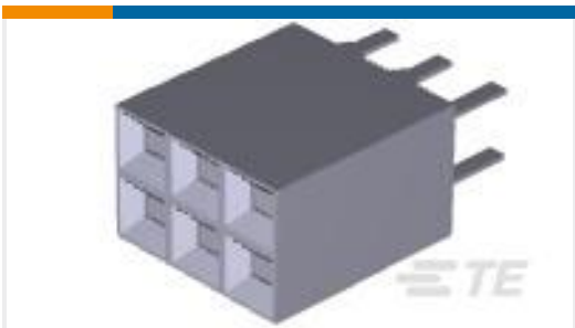
TE Part #640453-6 Polyester Right Angle PCB Header: 2.54mm, Unshrouded, MTA 100
