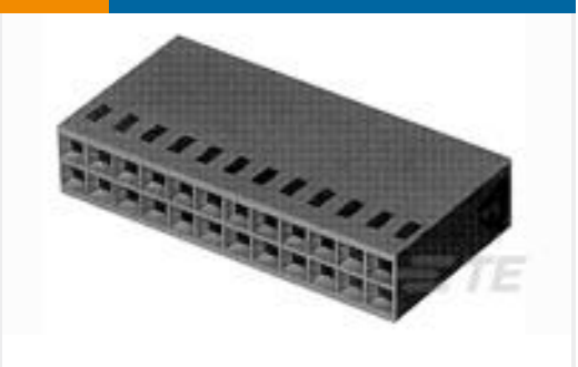
TE Part #1-87456-2 16 MODIV HSG DR MRKD .100CL
