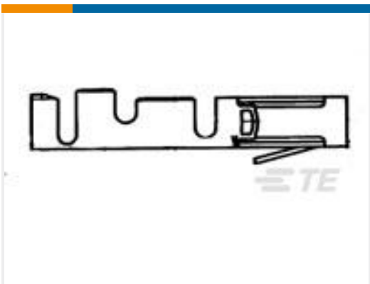
TE Part #182206-2 MOD 2 TERMINAL
