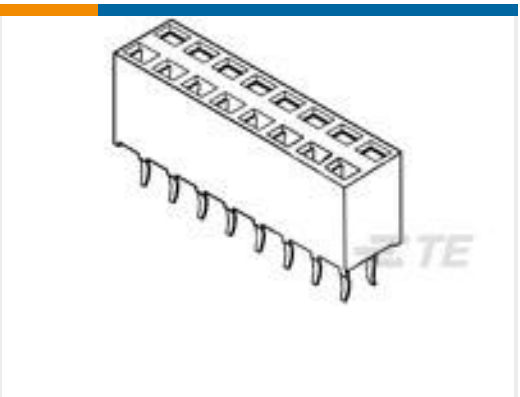
TE Part #215308-8 2X 8P HV100 REC CON. TE, 7.0MM, TIN
