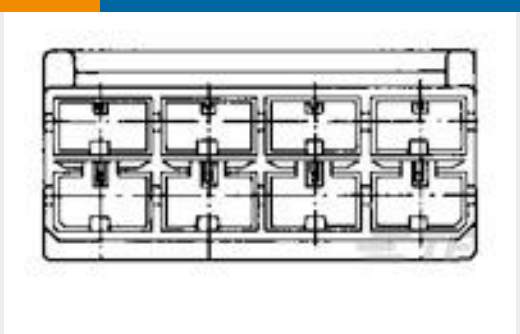
TE Part #926646-4 8P POS-LOCK GEH 6,3
