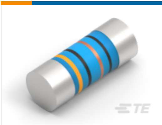
TE Part #2-2176334-1 MELF SMA-A 7K5 1% 50PPM 0204 0.4 W
