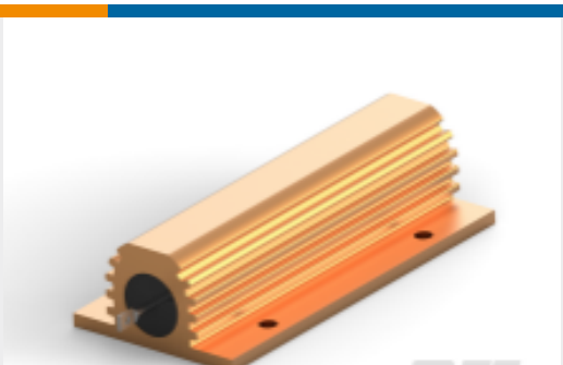
TE Part #1630027-3 Power Resistors: Aluminum Housed, HSC
