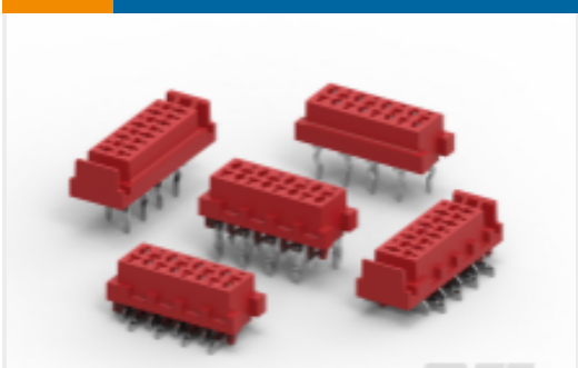
TE Part #2-100411-0 FEMALE-ON-BOARD CONNECTOR TOP ENTRY
