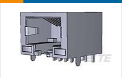
TE Part #1734324-1 RJ45,8P8C,w/ Y,G LED,shieled,dip,6u" Au
