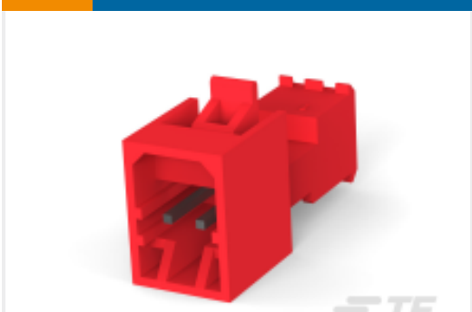
TE Part #3-647001-4 Nylon Tin Plated Plug: 2.54mm, With Mating Alignment, MTA 100
