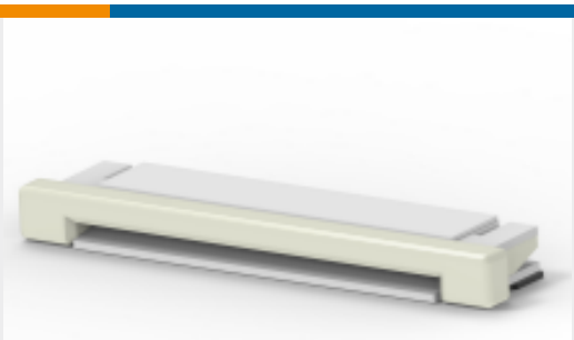
TE Part #1-1734742-2 0.5mm FPC Connectors
