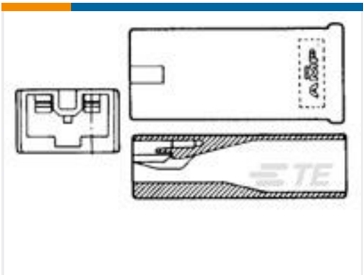
TE Part #179970-4 PL EXII 250 REC HSG 1P NYLON YELLOW
