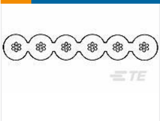
TE Part #2-57051-9 Madison Spec 100-7096 Rev. 3
